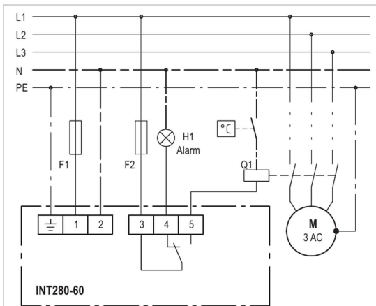
Wiring diagram
